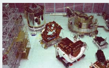
THE HUBBLE SPACE TELESCOPE CLEANROOM AT GODDARD SPACE CENTER IN GREENBELT, MD
