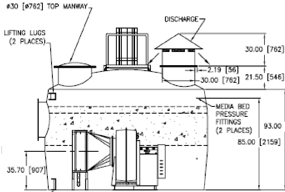
FIGURE 1: BASIC DESIGN OF SINGLE BED VESSEL SCRUBBER
